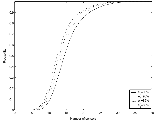
Figure 5: Probability that the minimum exposure is above e_d for varying number of sensors and e_d=80\%,85\%,90\% and 95\% .
