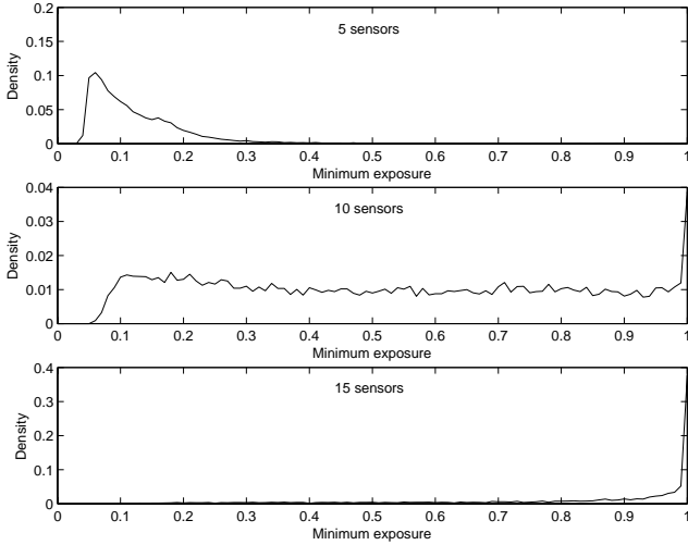
Figure 4: Probability density function for the distribution of minimum exposure for deployments of 5, 10 and 15 sensors.
