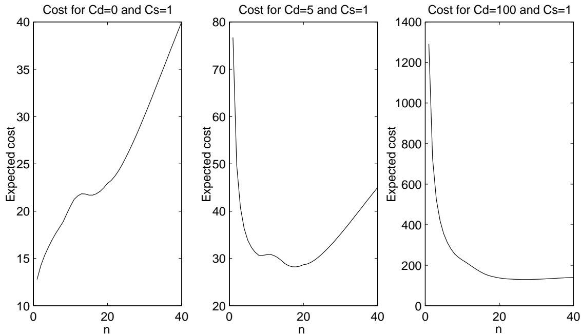
Figure 6: Expected cost of achieving minimum exposure of 95% as function of the number of sensors for three different cost assignments.
