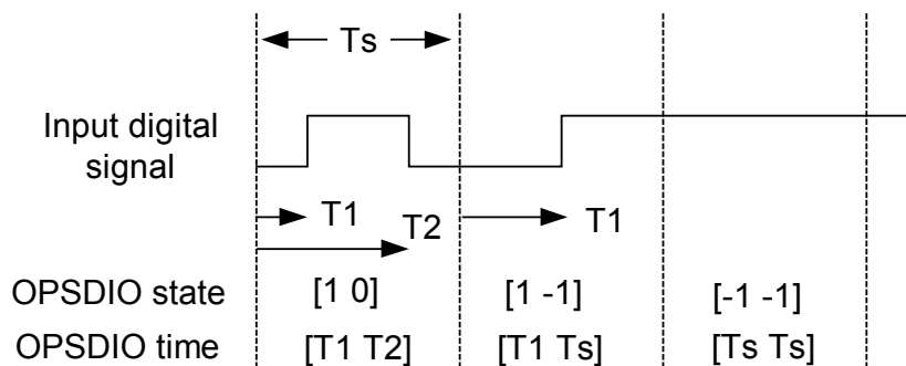
Fig. 6. OPSHDIO event format used in the matrix converter model
