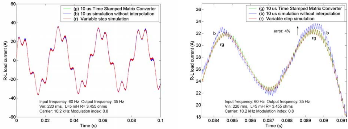
Fig. 8. Load current with details (right plot). No dead time
