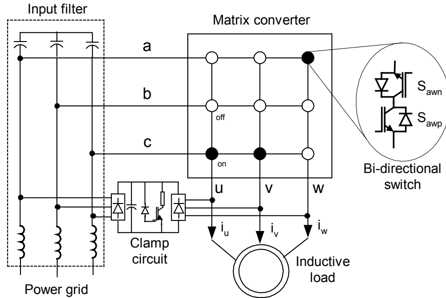
Fig. 1. Matrix converter with its input filter, load and clamp circuit.
