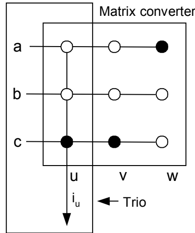
Fig. 7. The trio of IGBT pairs used for tests 1 & 2
