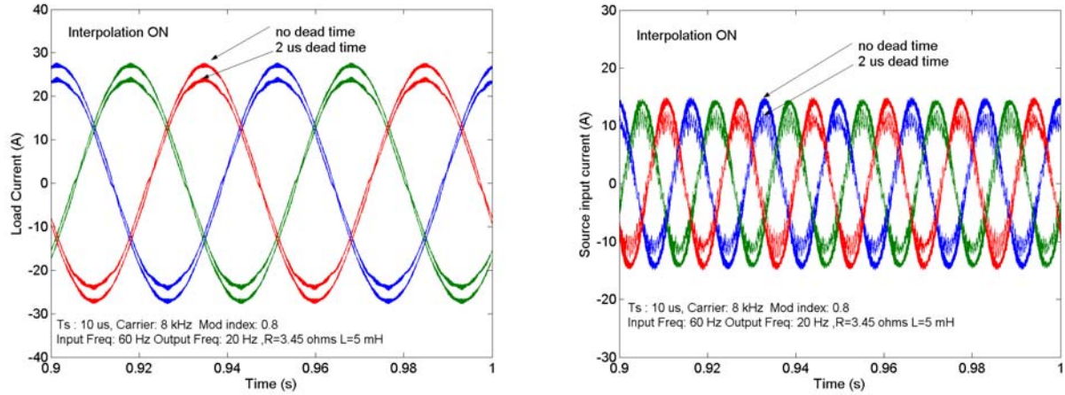
Fig. 10. Load current and filter input current with TSMC simulation at 10 \mu s time step
