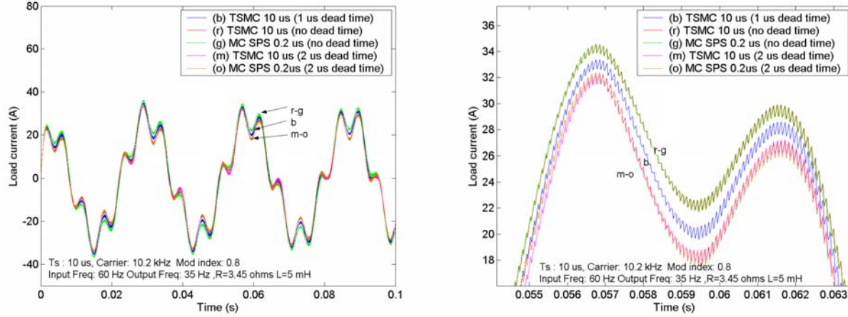
Fig. 9. Load current with deadtime
