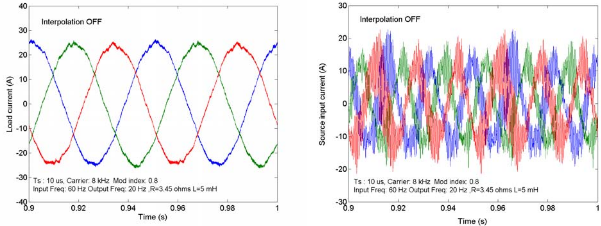
Fig. 11. Load and input filter current simulation at 10 \mu s time step with interpolation disabled
