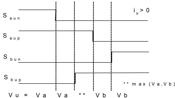
Fig. 5. Switching sequence to change the voltage of one phase of the load
