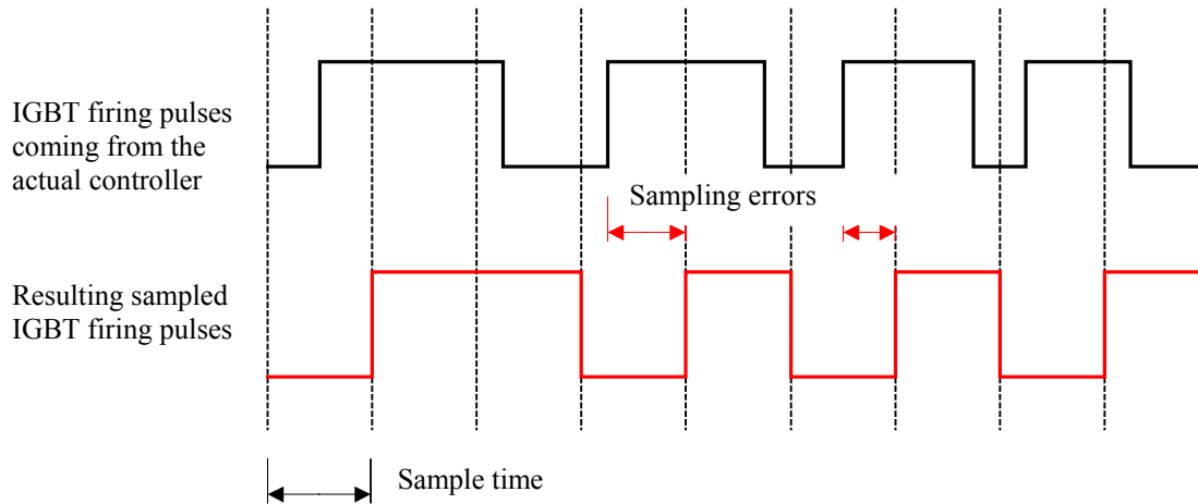
Fig. 2. Sampling errors made with standard I/O
