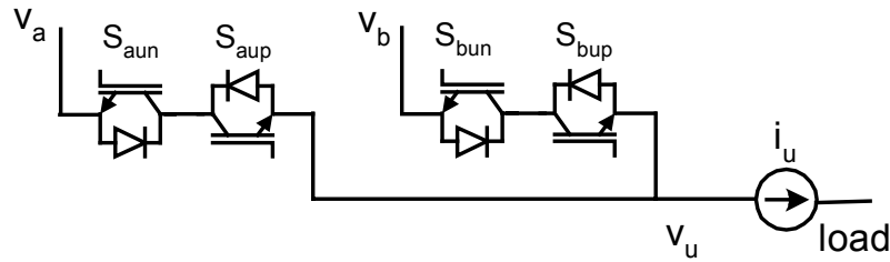
Fig. 4. Two pairs of switches of the matrix converter
