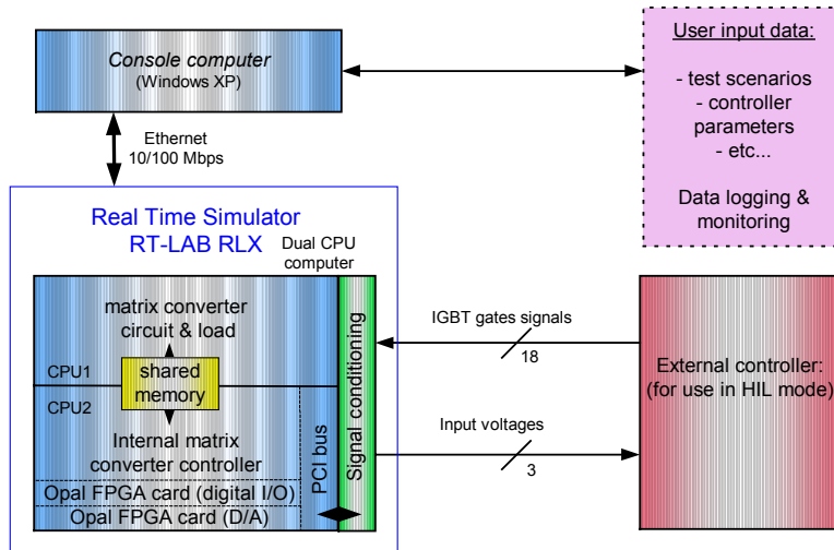
Fig. 3. Structure of the RT-LAB real-time simulator
